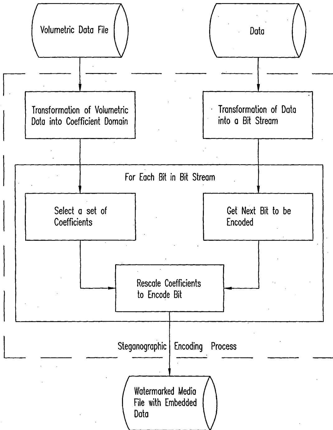
Encoding Data in a Volumetric Data File
